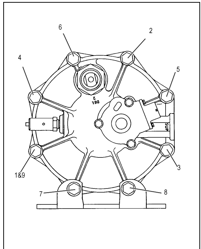
FIGURE 8 - END COVER TO HOUSING TORQUE PATTERN
