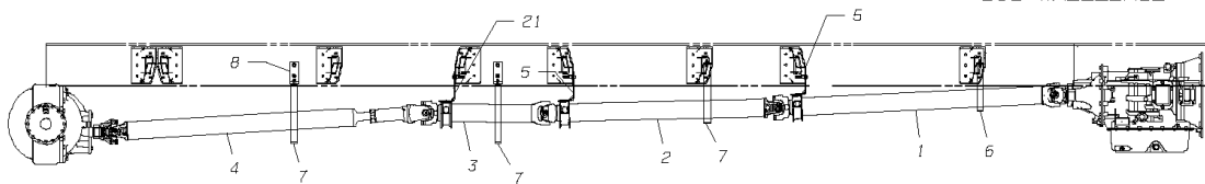
232 WHEELBASE
