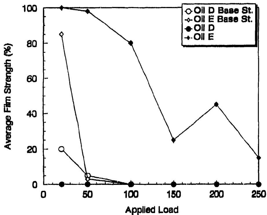
Figure 31. Average film strength for Oils D and E compared to their base stocks
