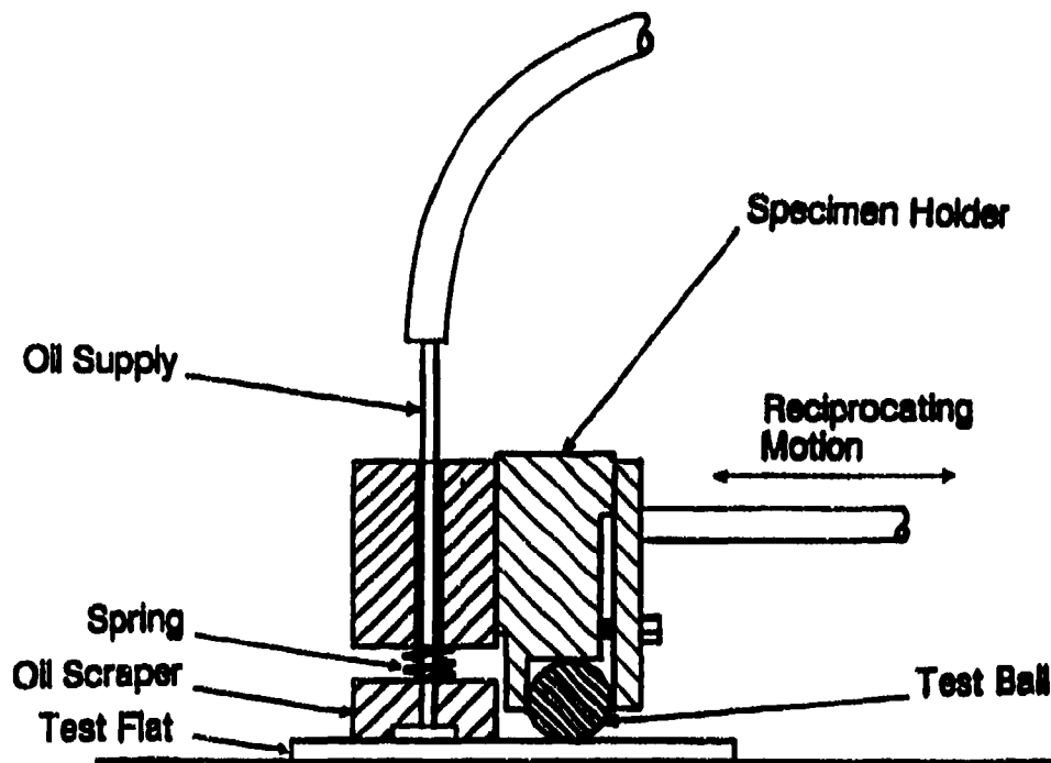
Figure 38. Schematic diagram of revised contact geometry/lubricant supply system used in high-temperature tests
