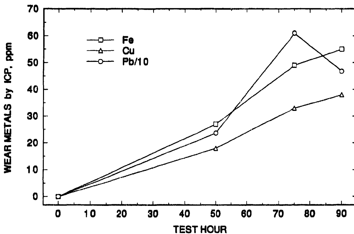
Figure 14. Test A-3, Oil C, wear metals
