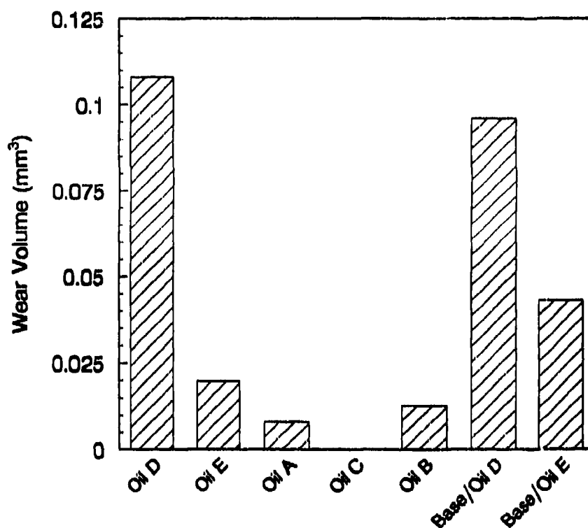
Figure 29. Wear tests with ring zone materials at 160°C
