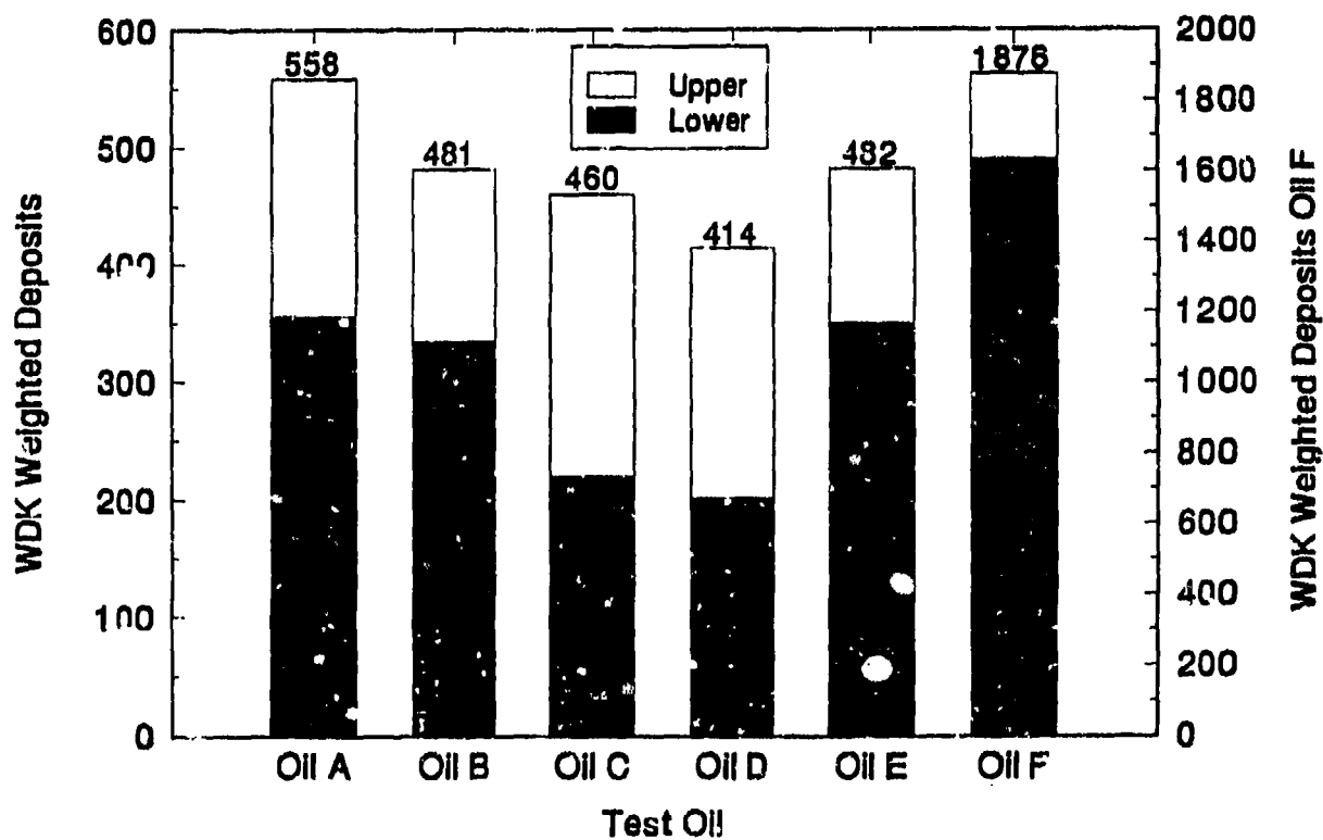
Figure 24. Grouped locational deposit ratings for pistons
