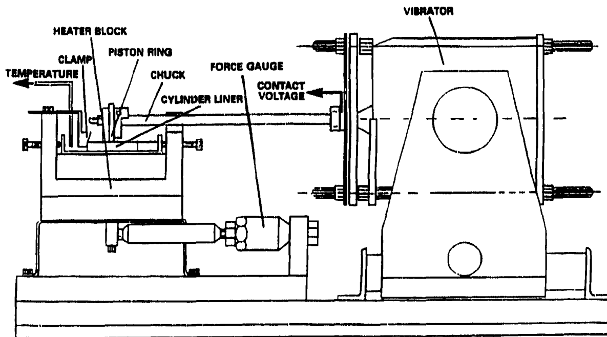
Figure 28. Schematic diagram of the Cameron-Plint test apparatus
