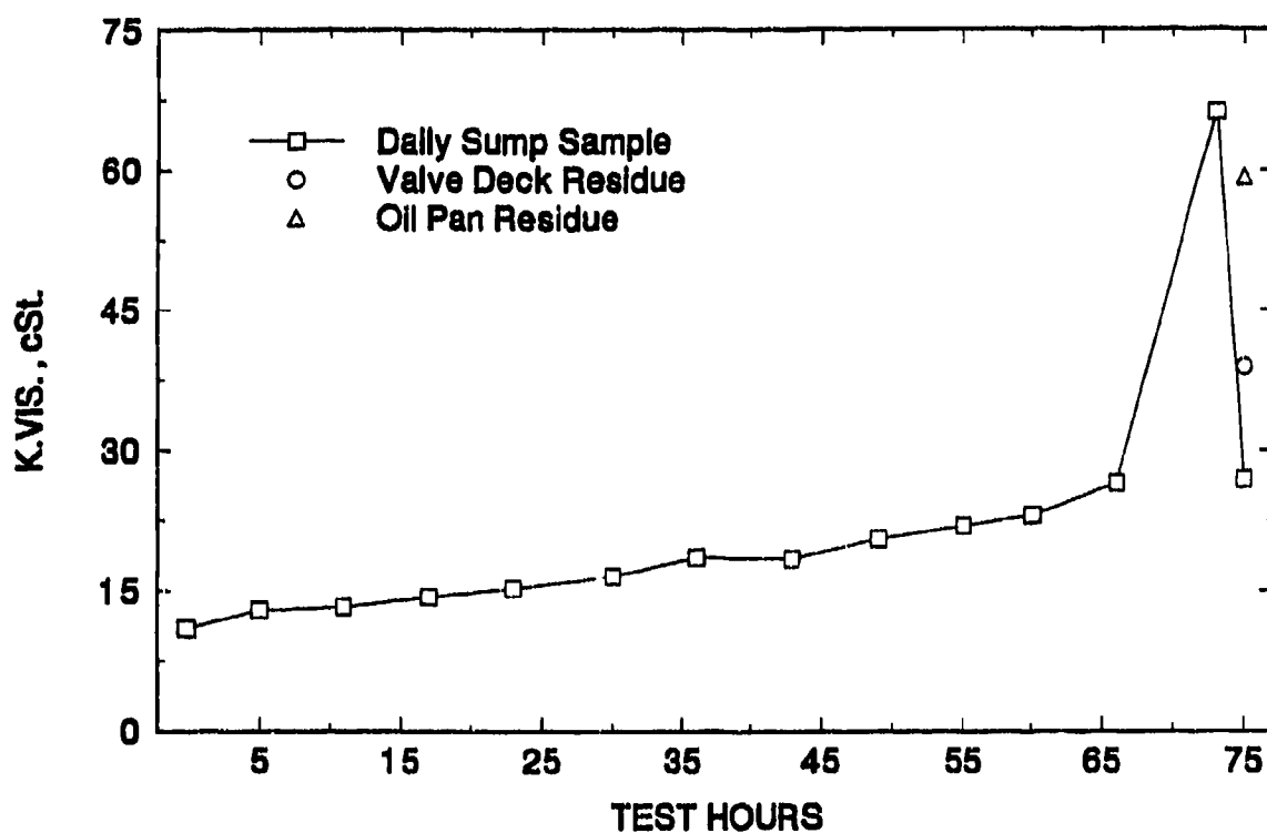
Figure G-2. AIPS-7, AL-19902, K. vis., 100°C
