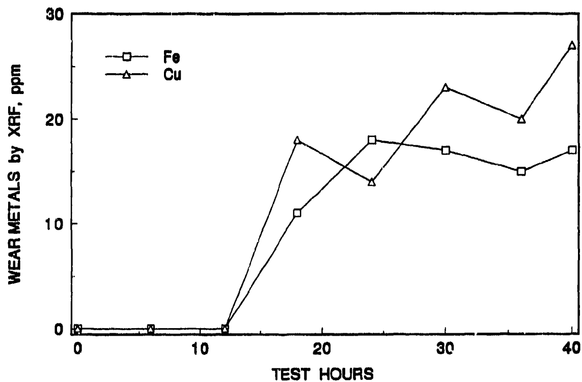
Figure 10. Test A-2, Oil B, wear metals
