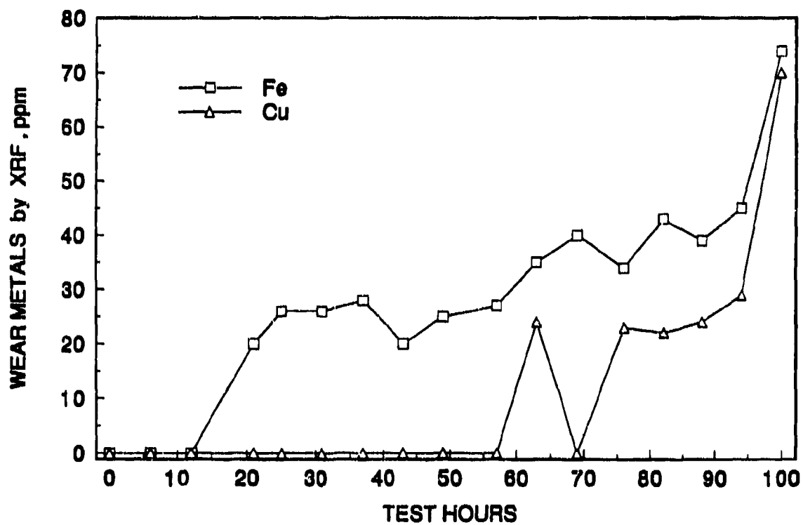
Figure 18. Test A-5, Oil E, wear metals
