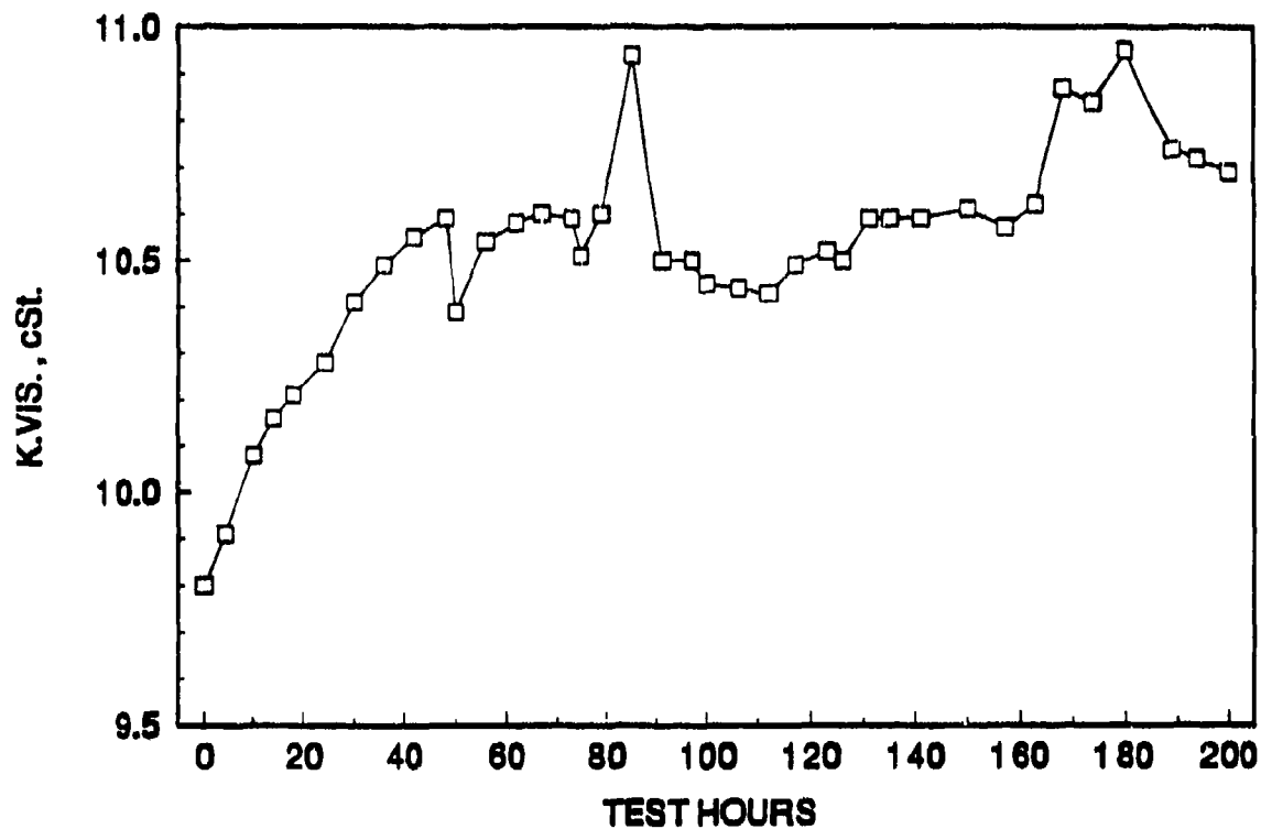
Figure 15. Test A-4, Oil D, K. Vis at 100°C
