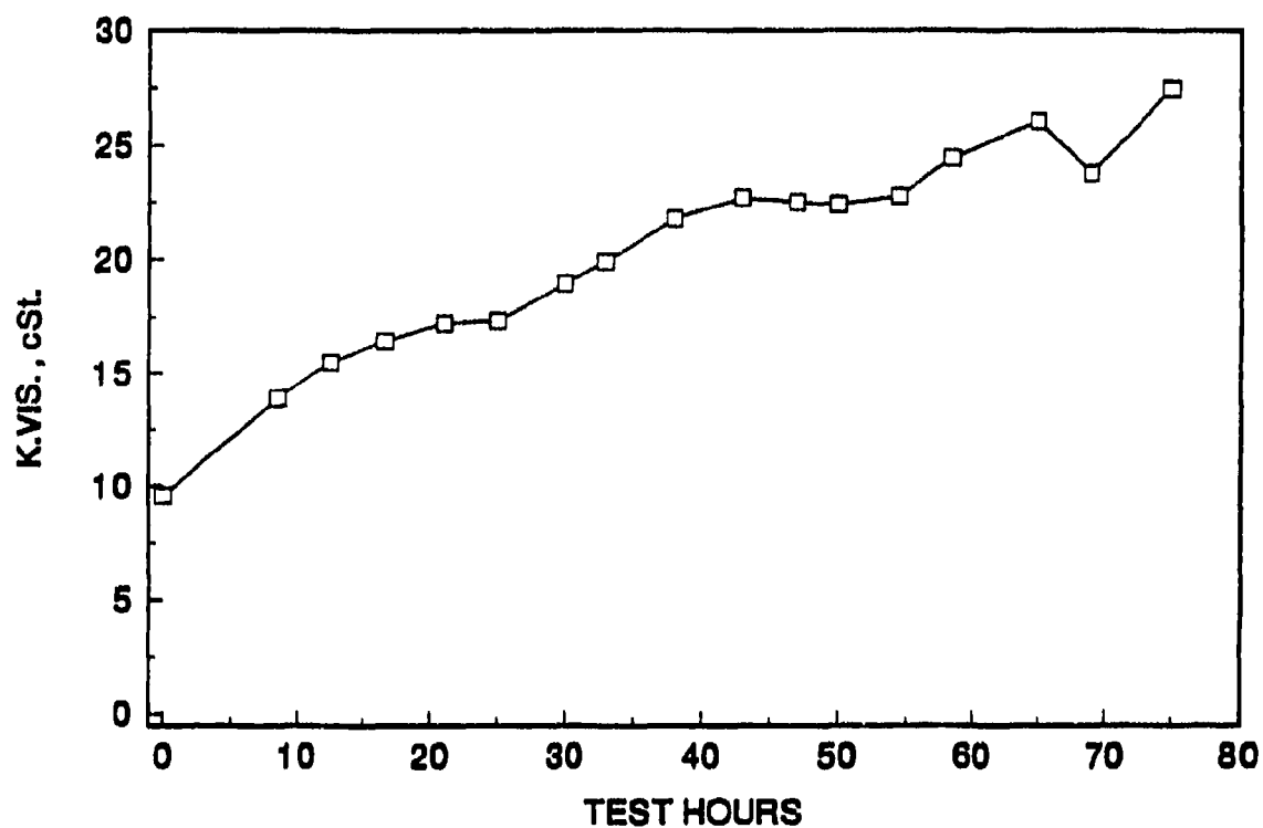
Figure 7. Test A-1, Oil A, K. Vls at 100°C
