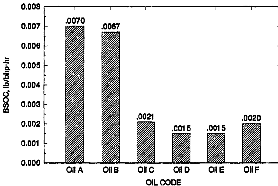
Figure 22. BSOC, lb/Bhp-hr
