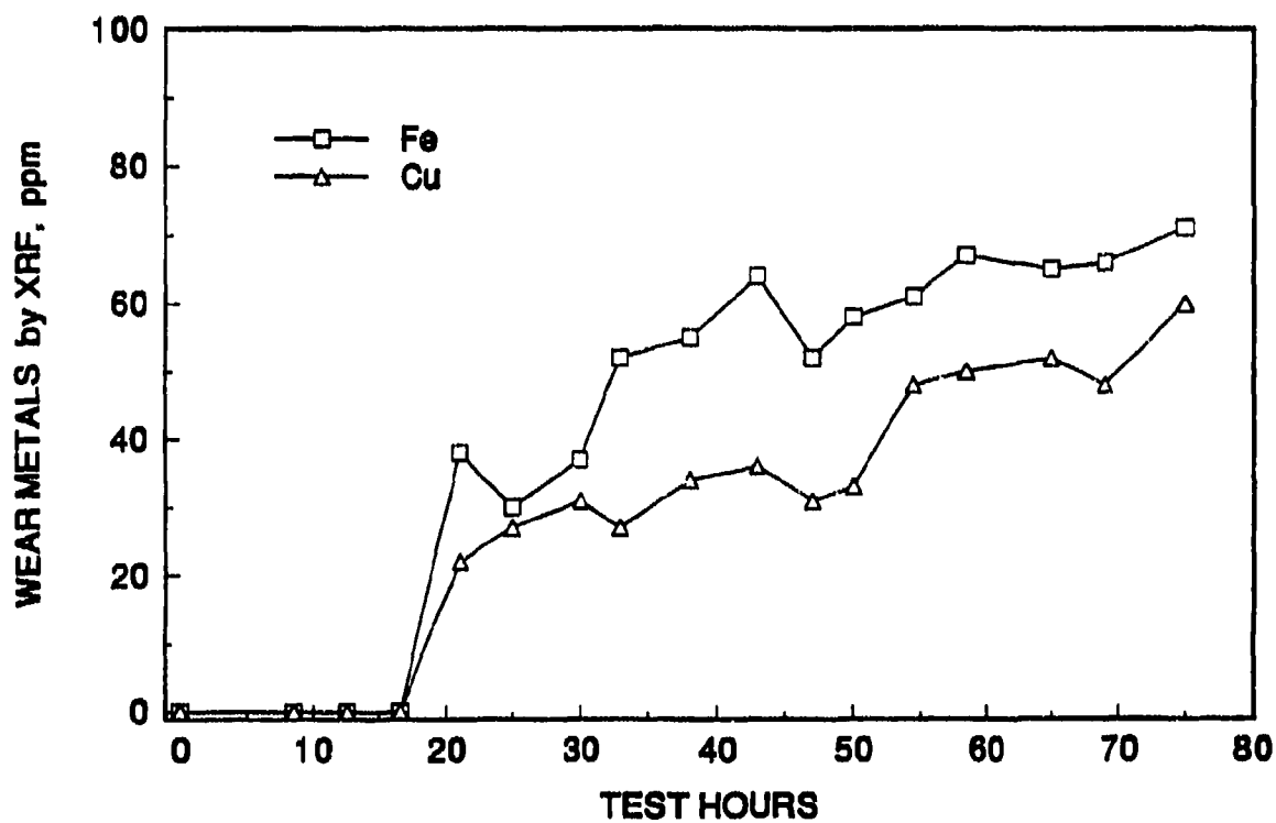
Figure 8. Test A-1, Oil A, wear metals
