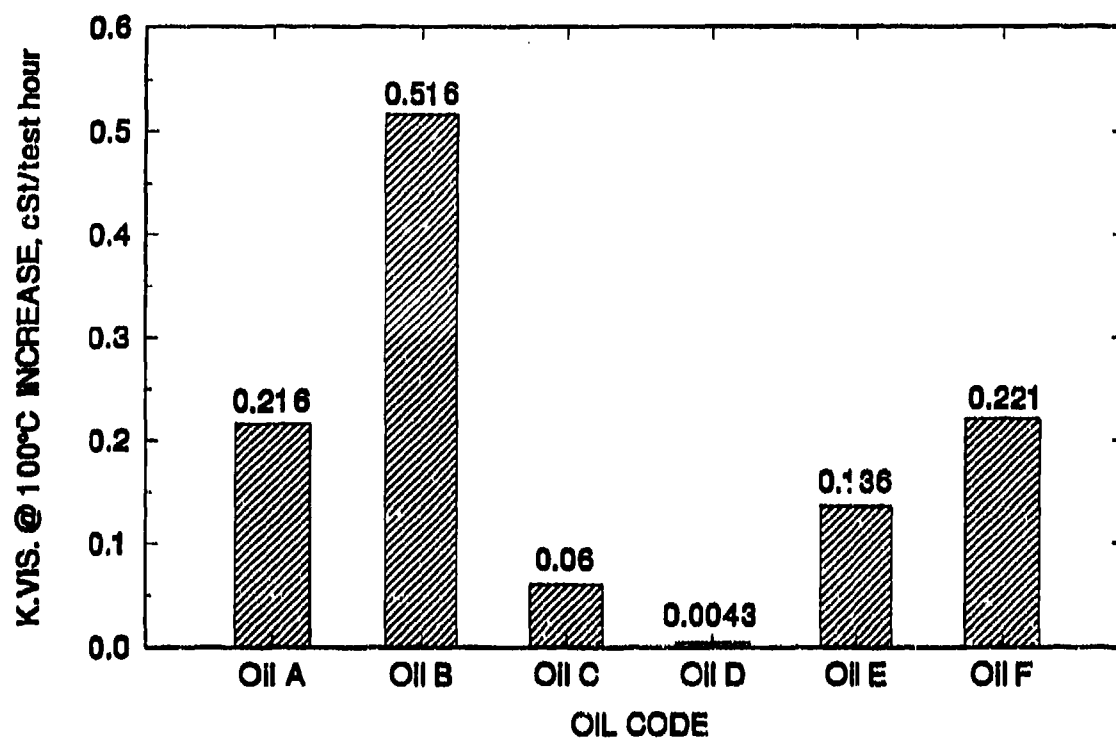
Figure 21. K. Vis at 100°C increase, cSt/test hour
