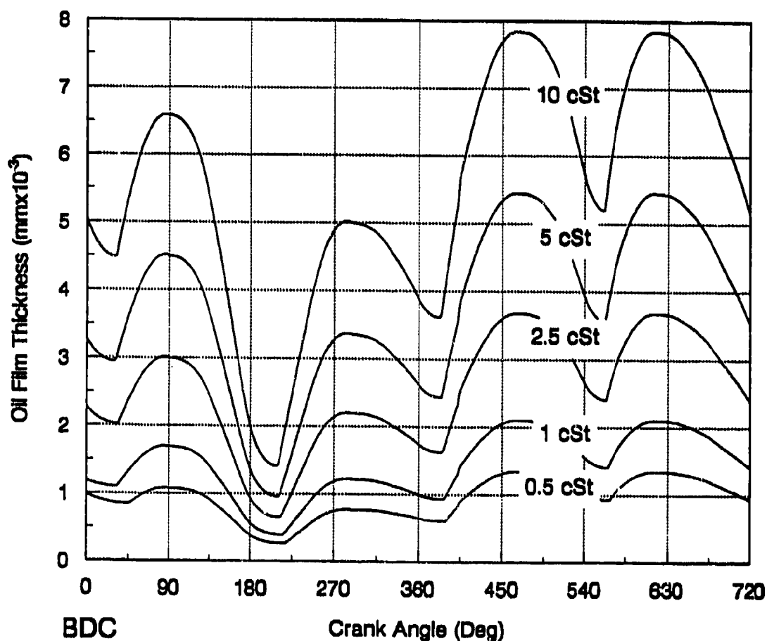
Figure 26. Theoretical oil film thickness throughout combustion cycle at 2200 rpm
