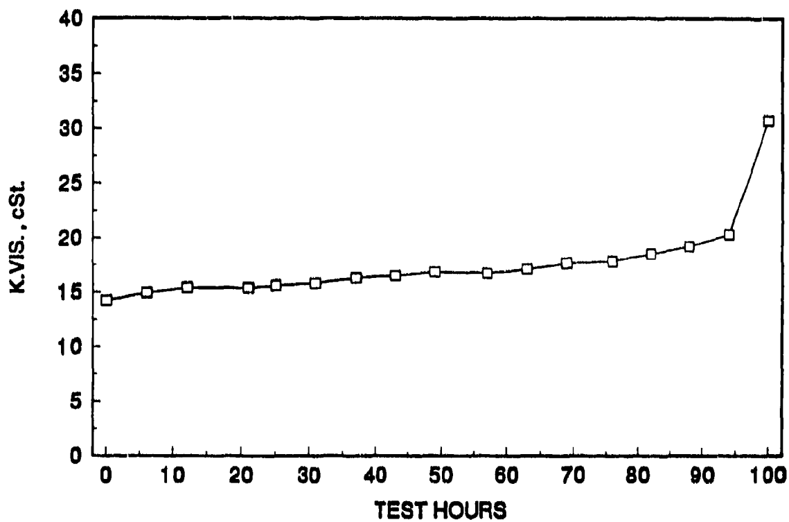
Figure 17. Test A-5, Oil E, K. Vls at 100°C
