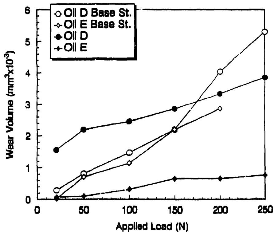
Figure 30. Wear volume for Oils D and E compared to their base stocks
