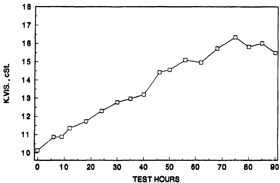
Figure 13. Test A-3, Oil C, K. Vis at 100°C
