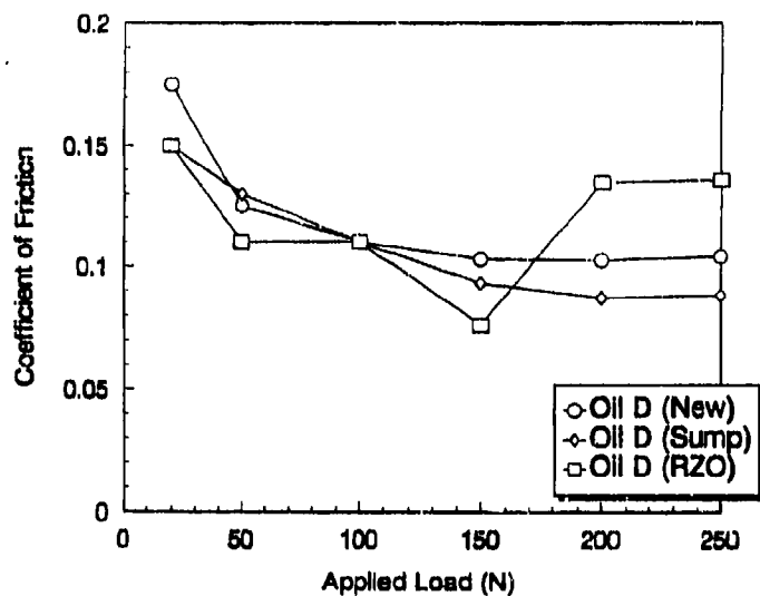
Figure 34. Comparison of new and used Oil D
