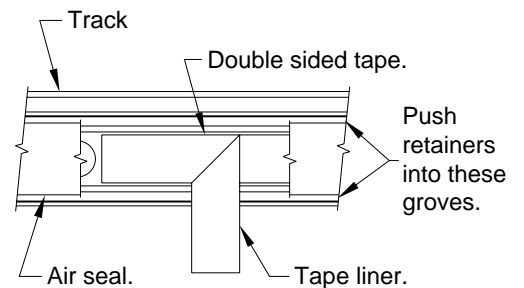
DETAIL H
