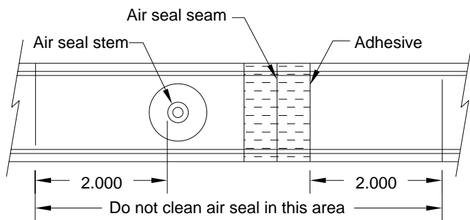
DETAIL G
