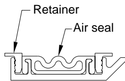
DETAIL D
