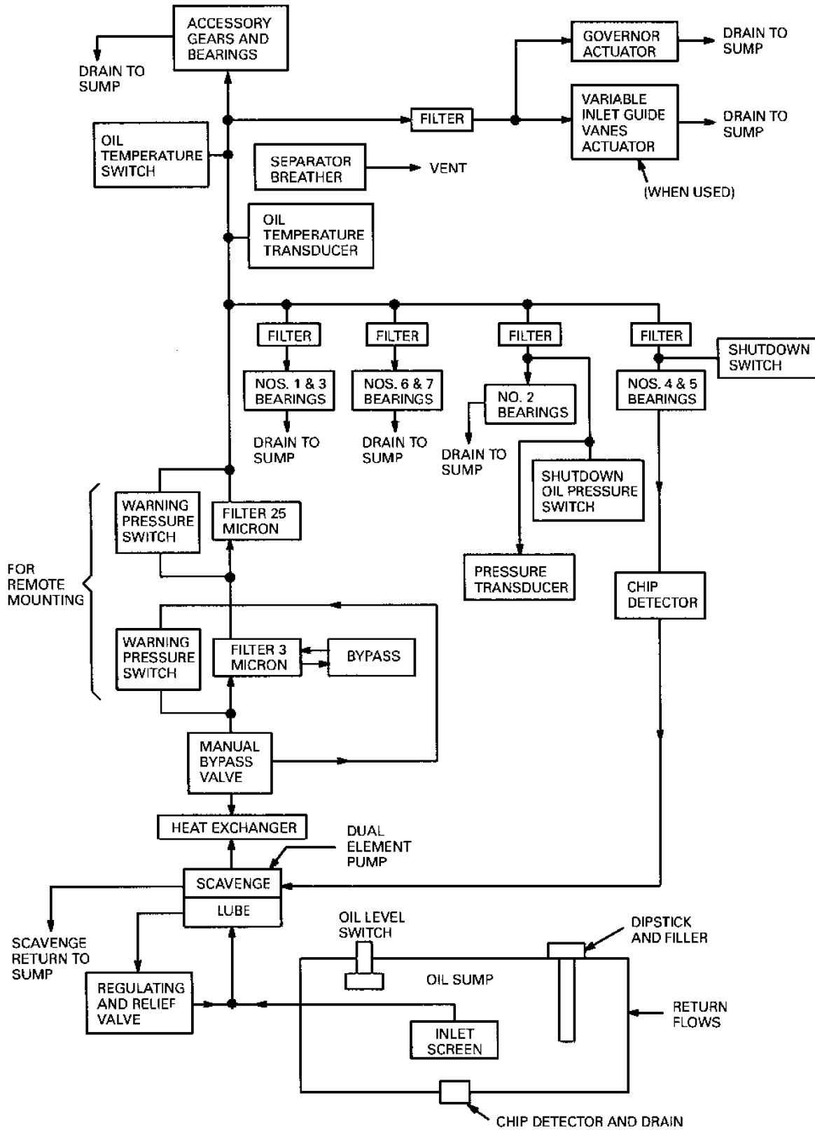
Figure 262-3-1. Simplified Schematic of Gas Turbine Internal Lubrication System
