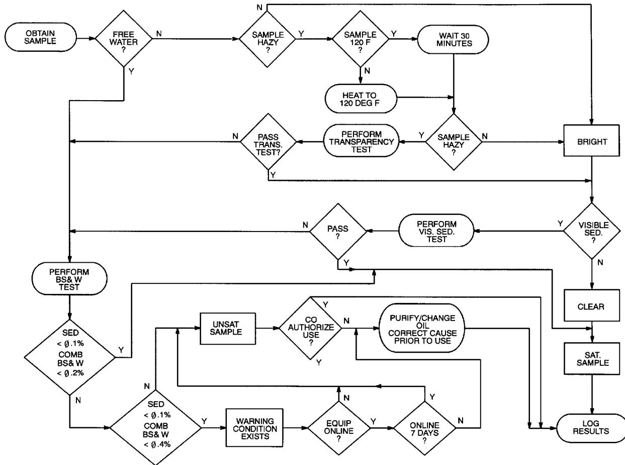
Figure 262-5-2. Flowchart for Systems Without Online Purification Capability
