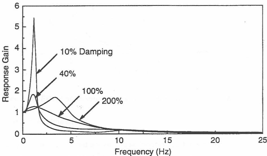
Figure 1.9: Effect of damping on suspension isolation behaviour [6].
