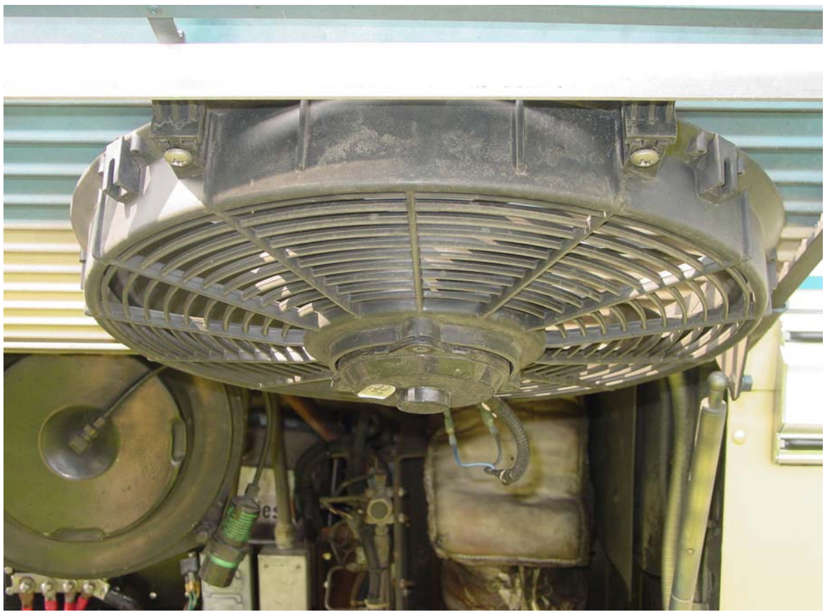
Photo # 3 Description: Close-up view of fan installation
